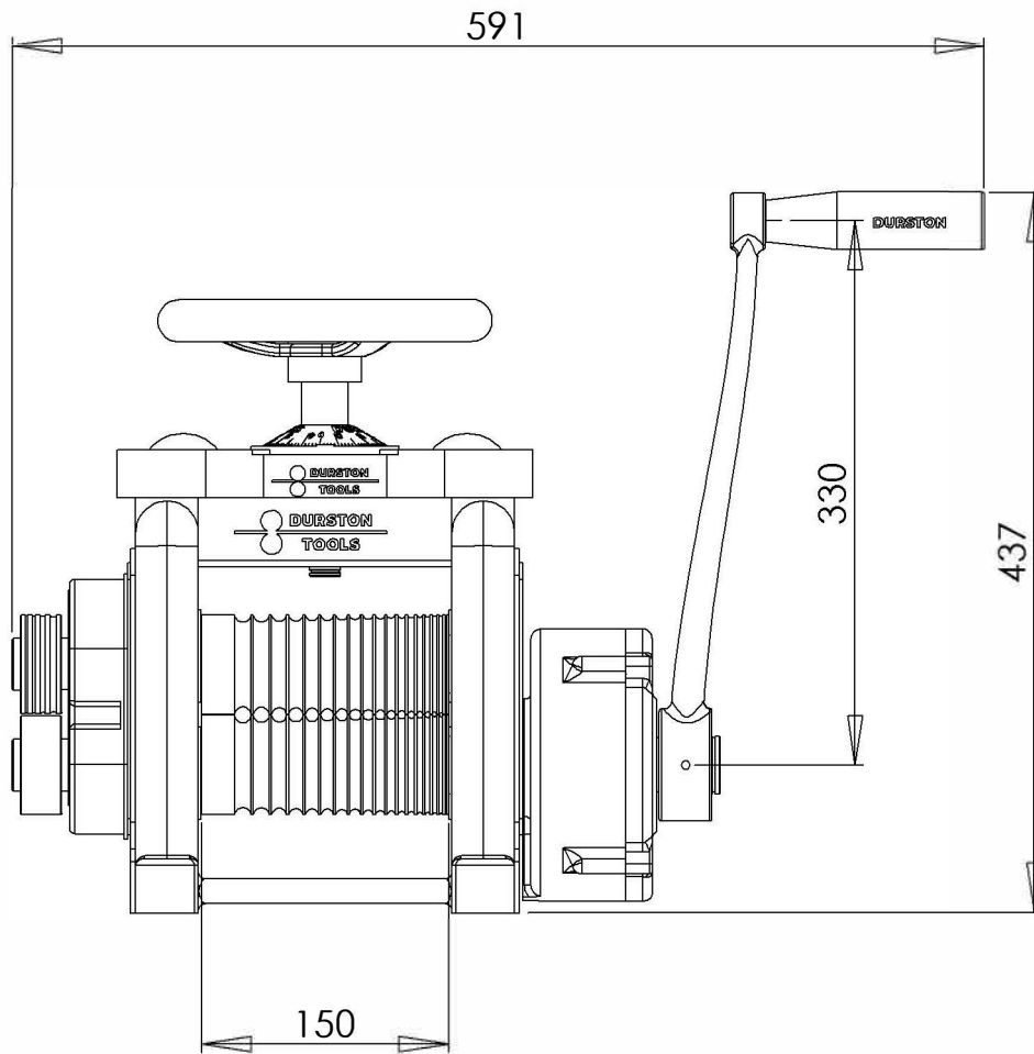
DRM 150RE Rolling Mill SKU: 1045 Dimensions in MM
