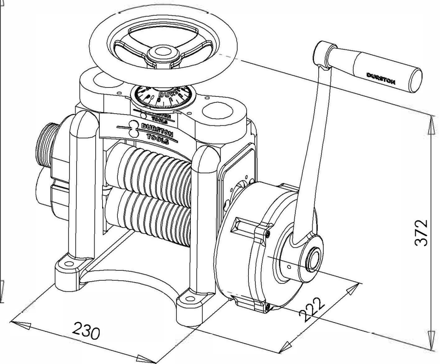
DRM 150RE Rolling Mill SKU: 1045 Dimensions in MM
