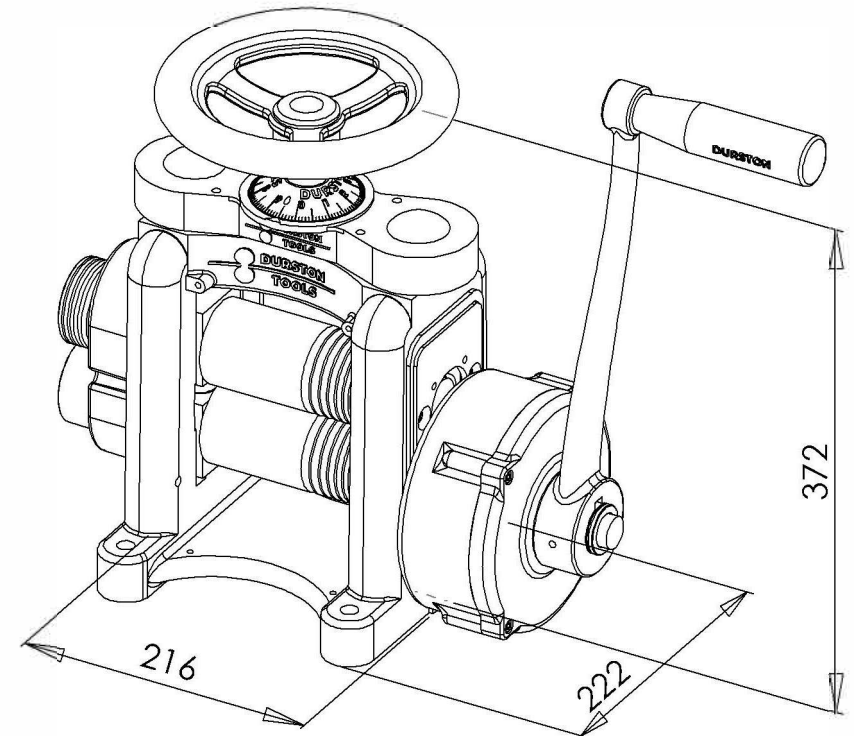
DRM Round 130RE Rolling Mill SKU: 1044 Dimensions is MM
