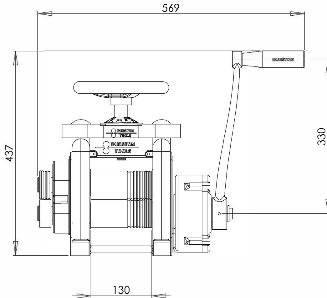
DRM Round 130RE Rolling Mill SKU: 1044 Dimensions is MM
