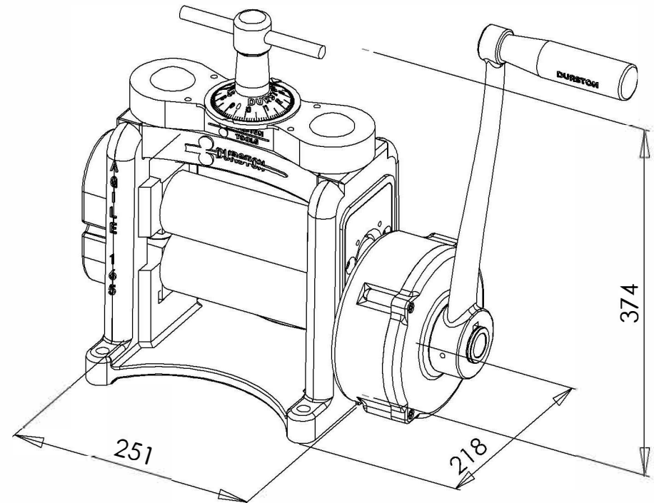
Agile F165 Rolling Mill SKU: 1040 Dimensions in MM
