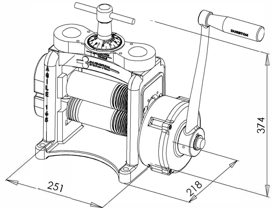
Agile C165 Rolling Mill SKU: 1039 Dimensions in MM
