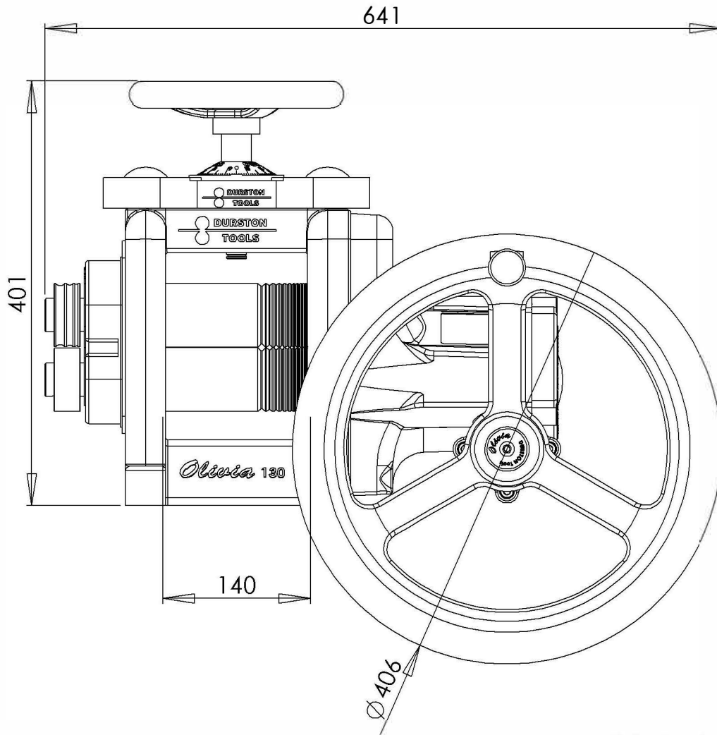
Olivia C130 Rolling Mill SKU: 1035 Dimensions is MM
