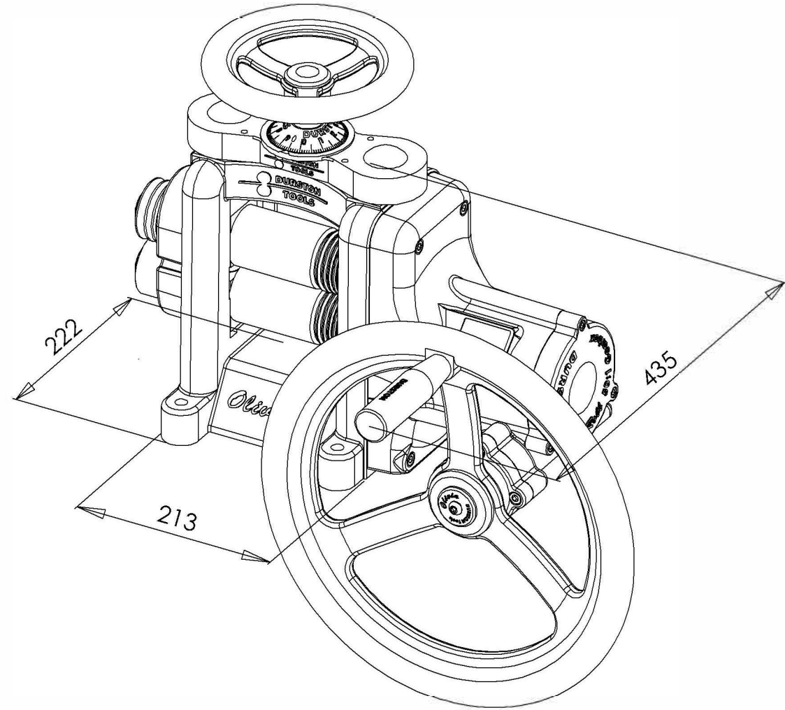
Olivia C130 Rolling Mill SKU: 1035 Dimensions is MM
