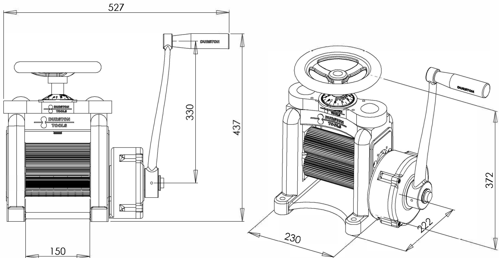
DRM Corrugated 150 Rolling Mill SKU: 1034 Dimensions is MM
