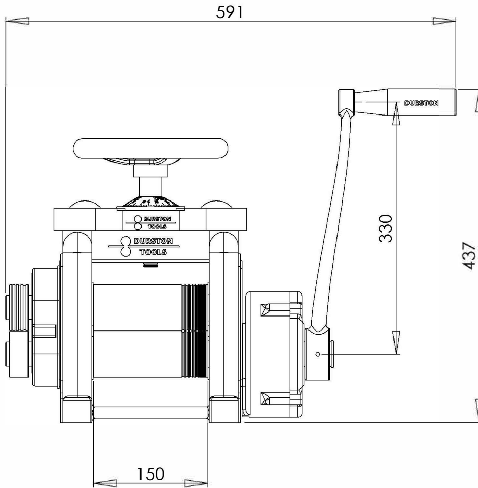
DRM C150RE Rolling Mill SKU: 1031 Dimensions in MM
