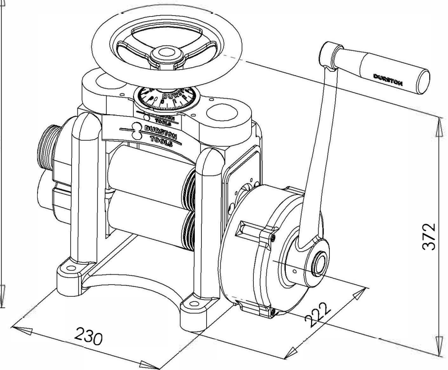
DRM C150RE Rolling Mill SKU: 1031 Dimensions in MM
