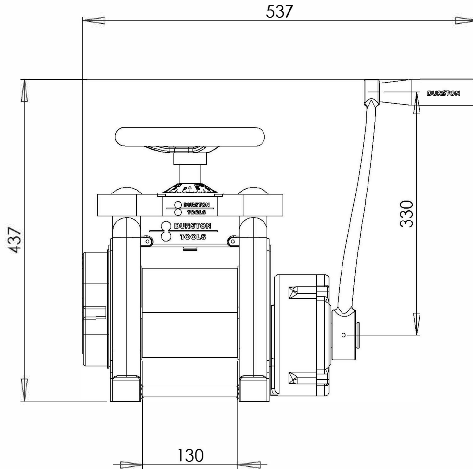
DRM F130R Rolling Mill SKU: 1026 Dimensions in MM
