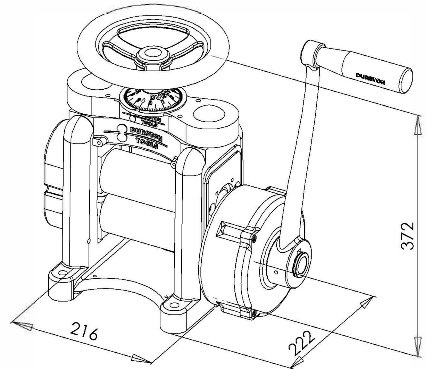
DRM F130R Rolling Mill SKU: 1026 Dimensions in MM
