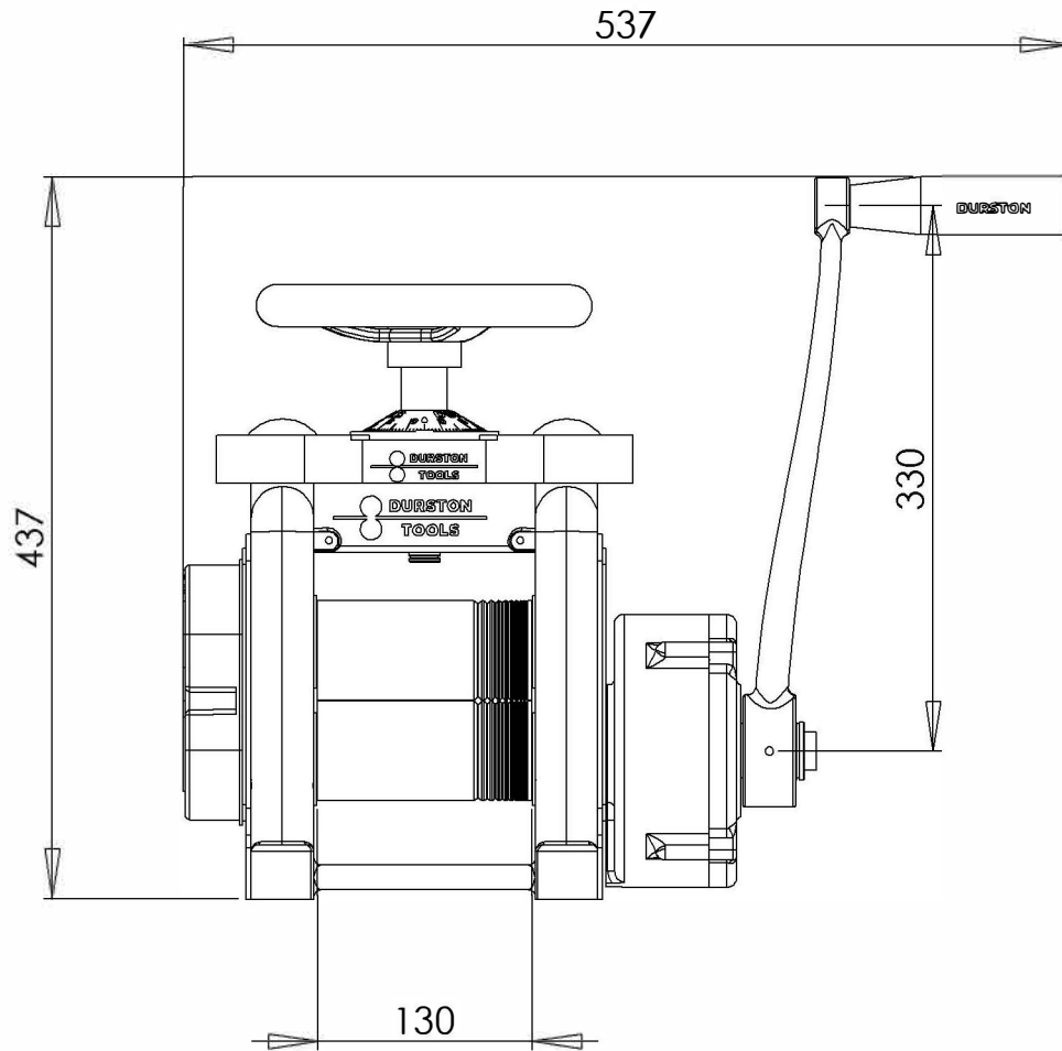
DRM C130R Rolling Mill SKU: 1025 Dimensions is MM
