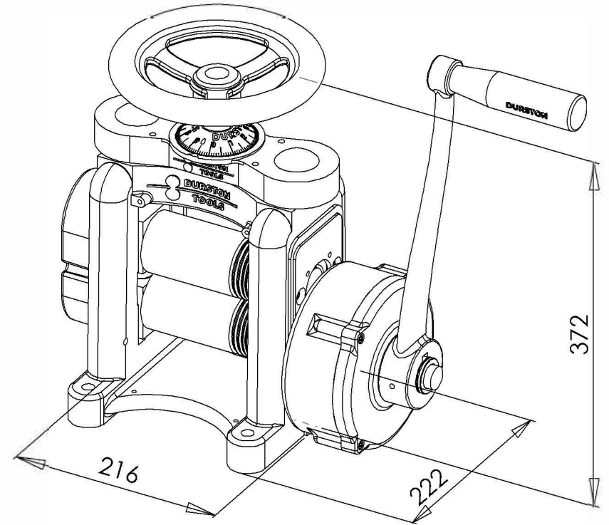
DRM C130R Rolling Mill SKU: 1025 Dimensions is MM
