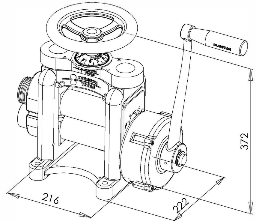
DRM F130RE Rolling Mill SKU: 1023 Dimensions is MM
