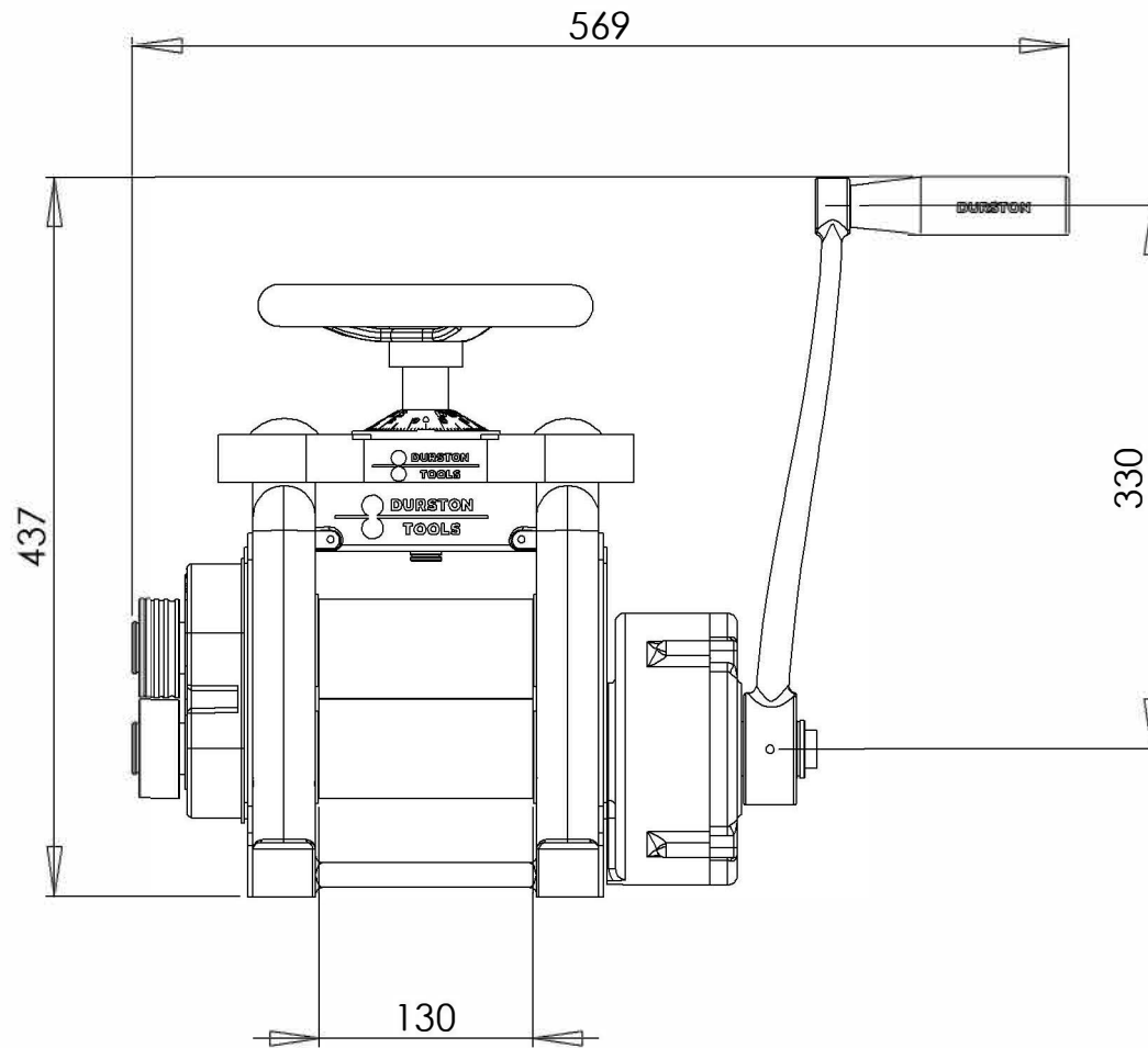
DRM F130RE Rolling Mill SKU: 1023 Dimensions is MM
