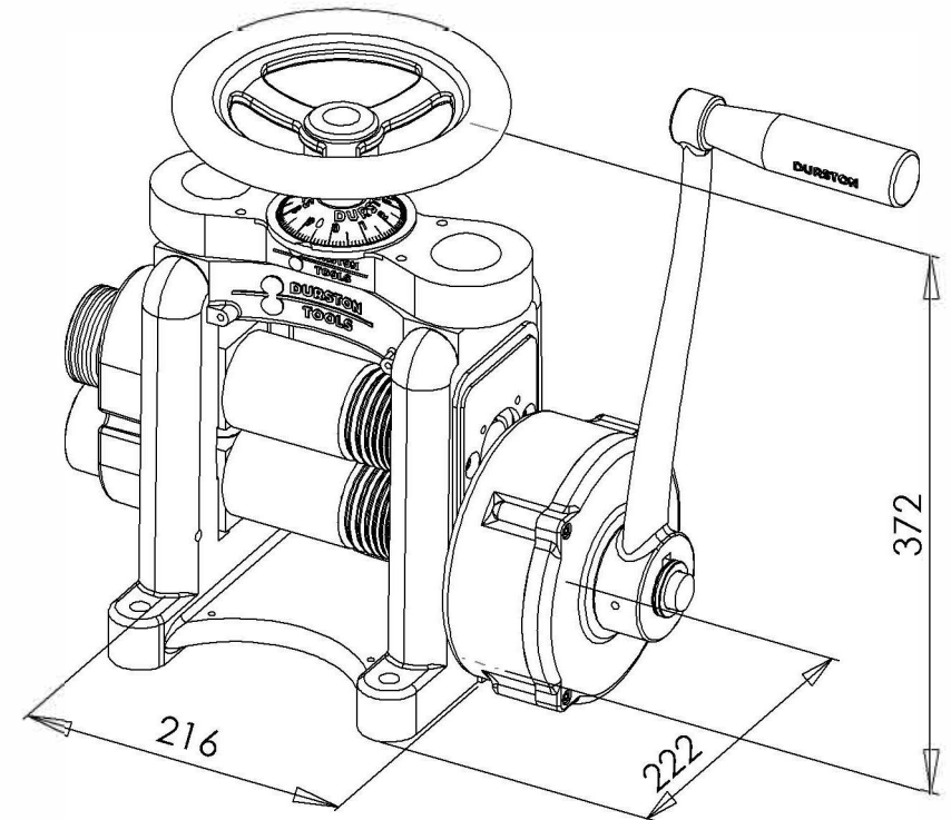
DRM C130RE Rolling Mill SKU: 1021 Dimensions is MM
