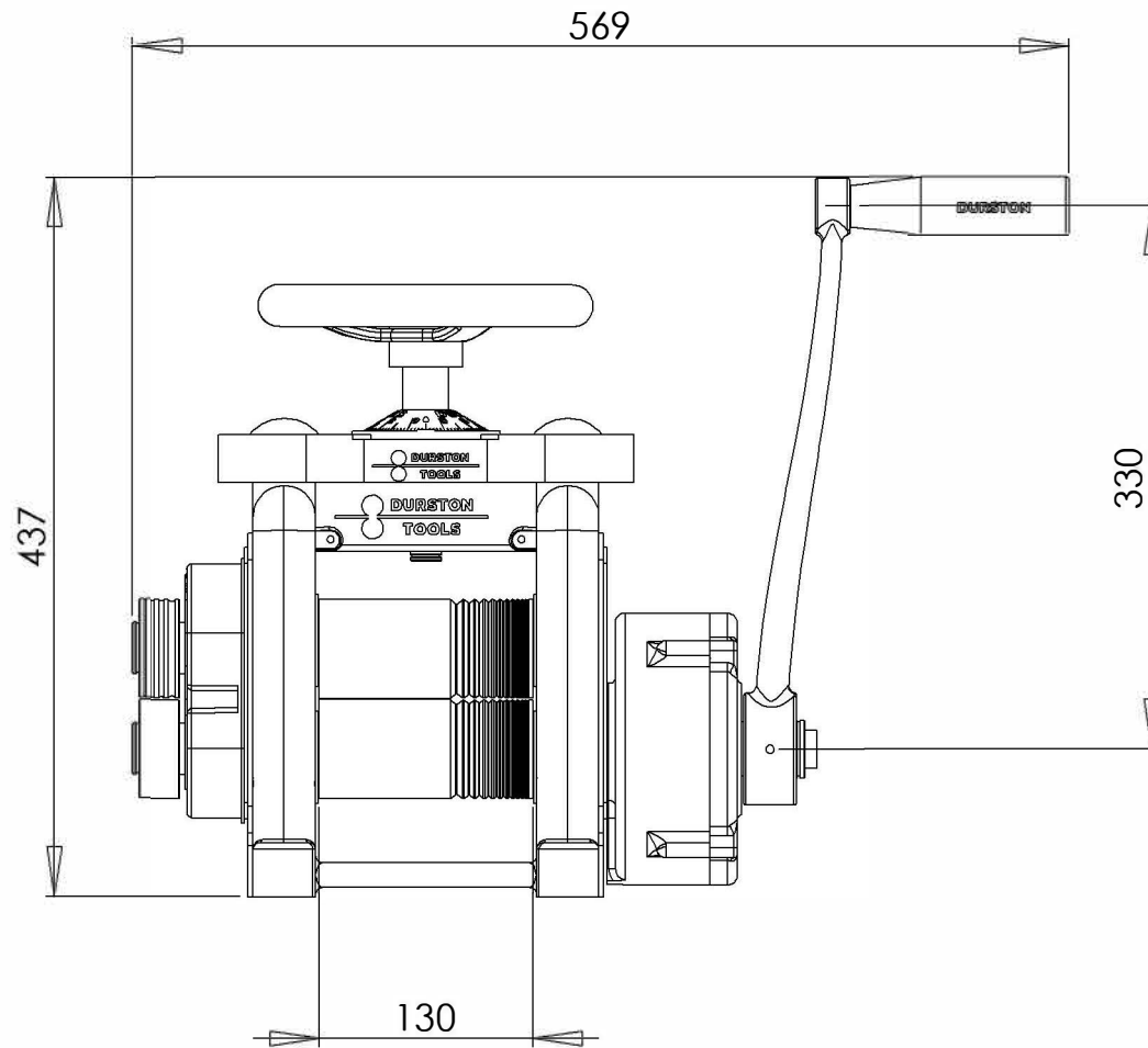
DRM C130RE Rolling Mill SKU: 1021 Dimensions is MM
