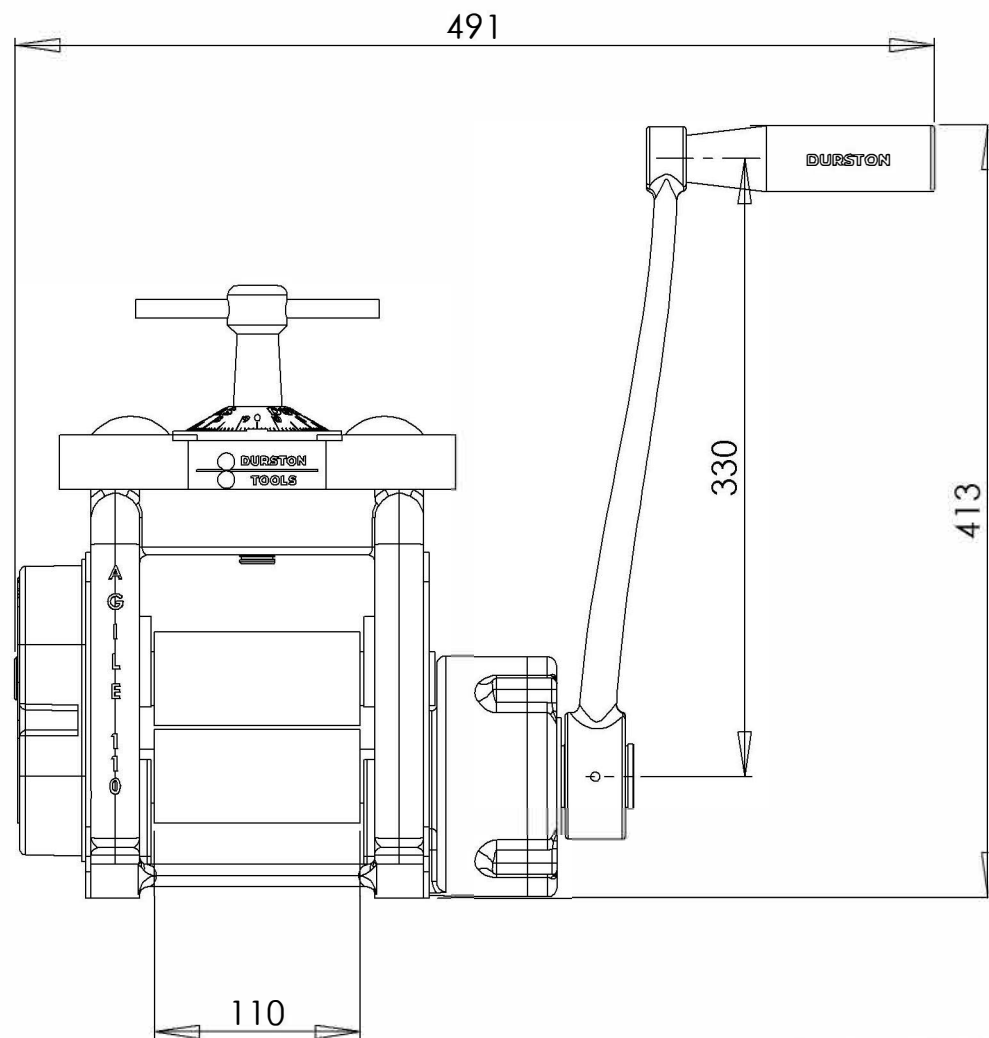
Agile F110 Rolling Mill SKU: 1020 Dimensions is MM
