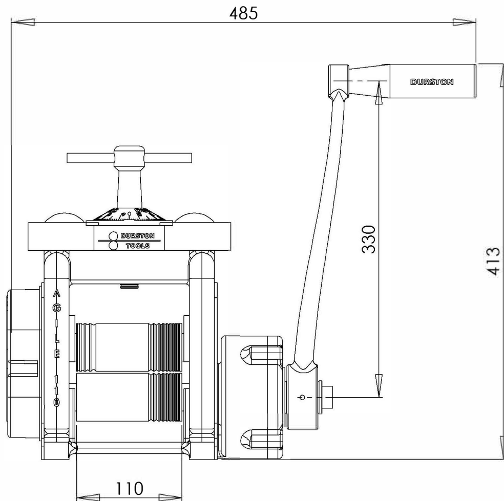
Agile C110 Rolling Mill SKU: 1019 Dimensions in MM
