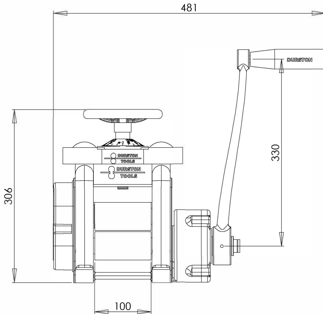
DRM F100R Rolling Mill SKU: 1016 Dimensions is MM
