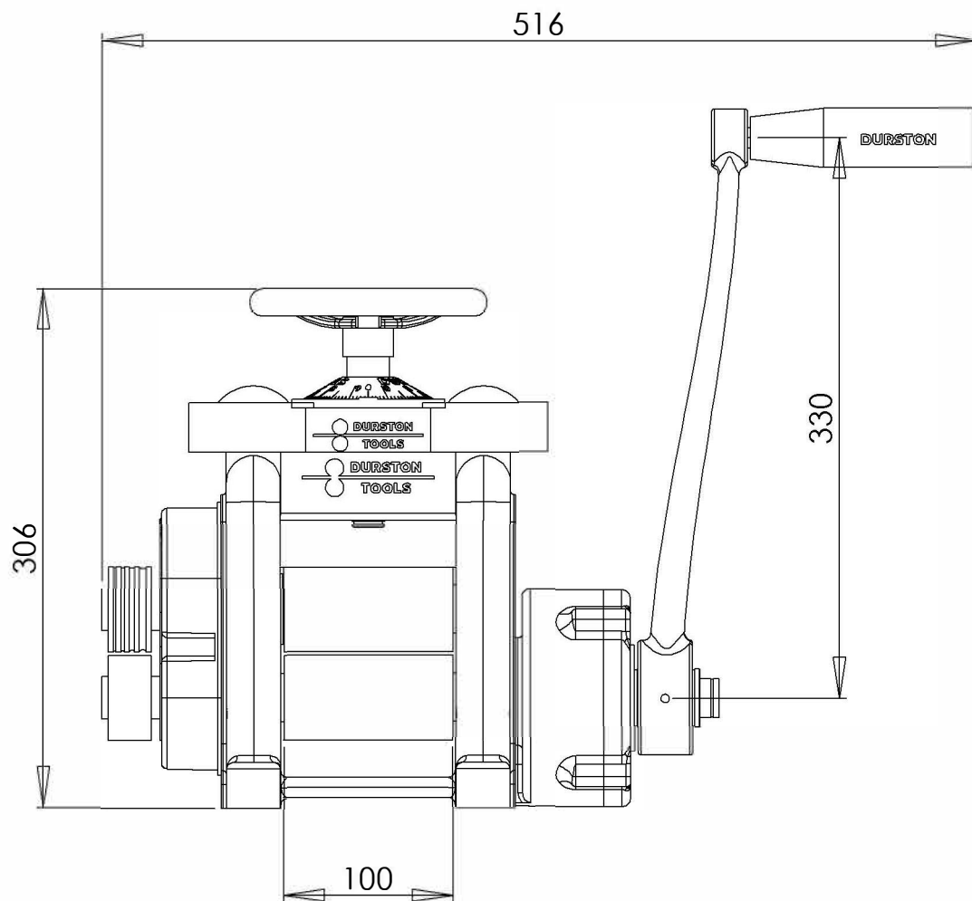
DRM F100RE Rolling Mill SKU: 1013 Dimensions in MM
