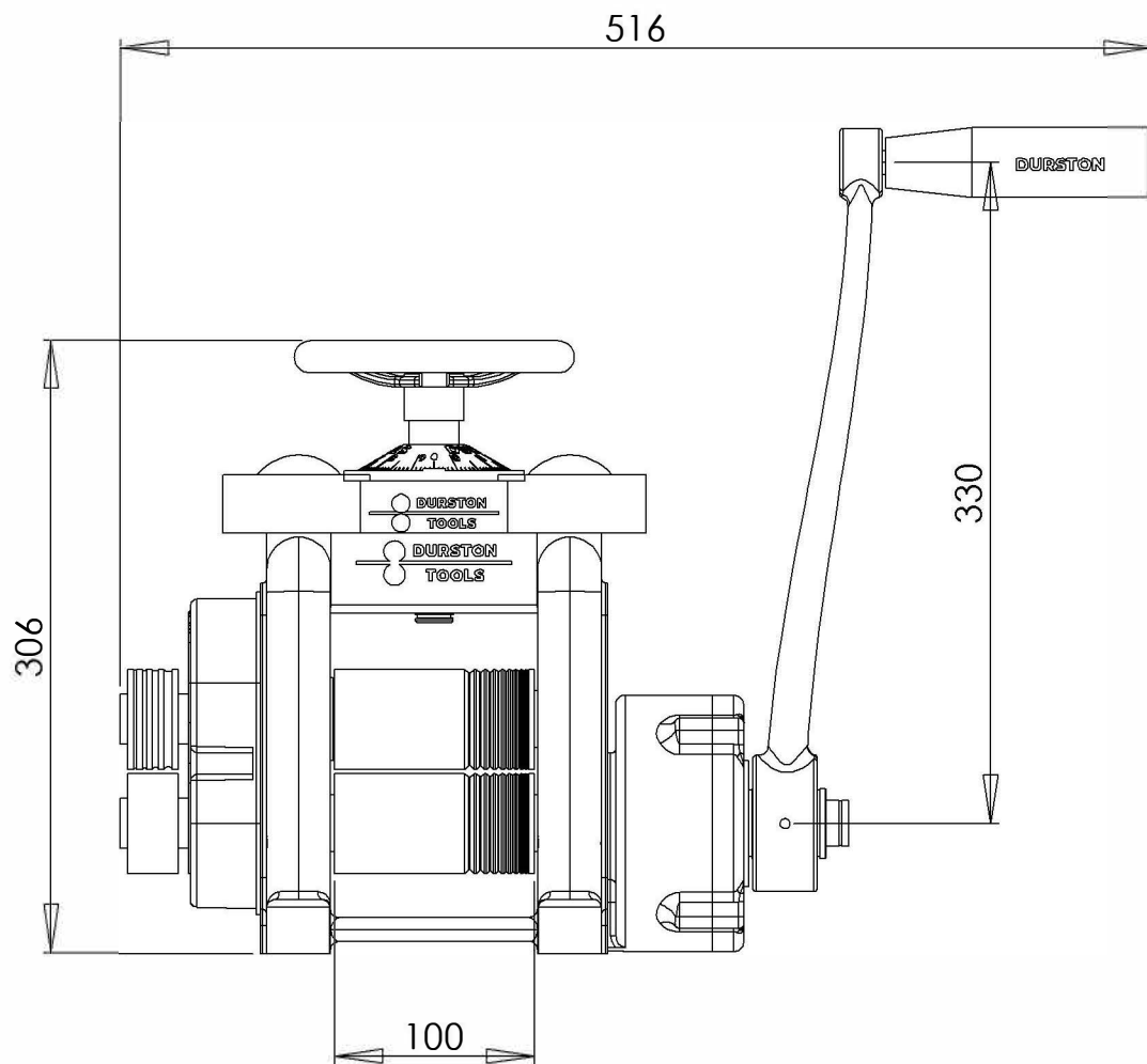
DRM C100RE Rolling Mill SKU: 1011 Dimensions in MM
